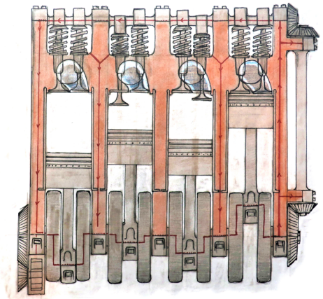
Engine Drawing - 2023
