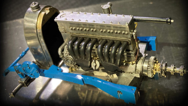
1. Bugatti Type 35 Engine
