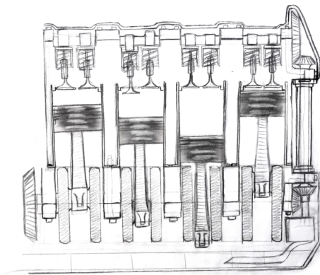
Engine Drawing - 2023
