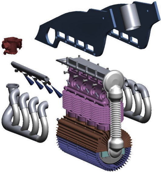
Engine As Structural Member CAD - 2023
