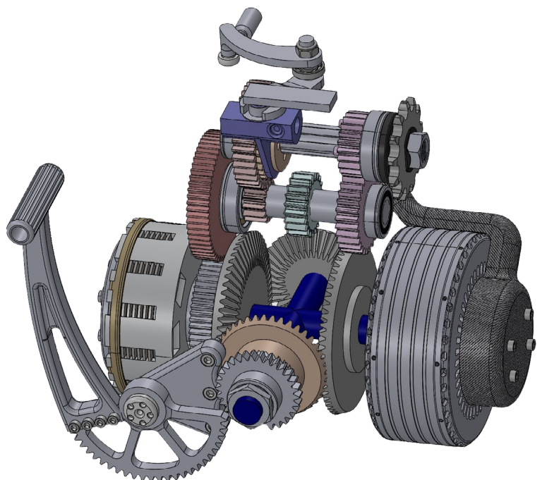
Kickstarter with Axial Flux Mag Dyno
