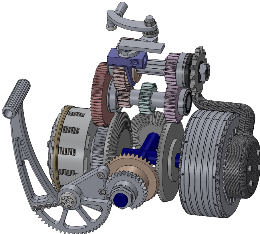
Transmission Drawing - 2023
