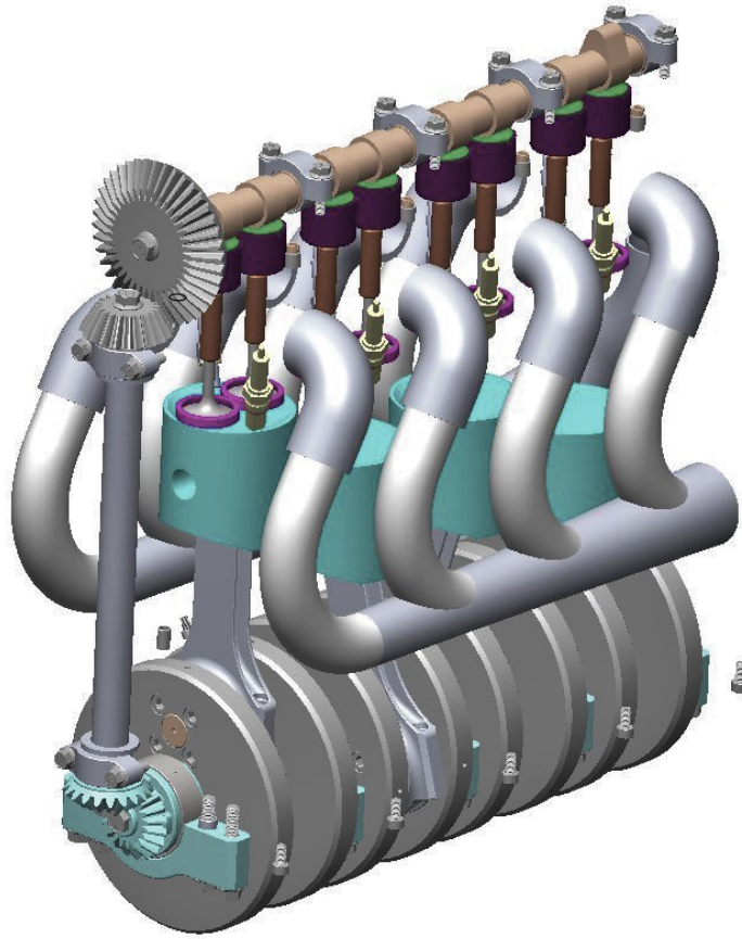
Camshaft Valve Configuration
