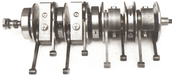
Bugatti Type 35 Crankshaft
