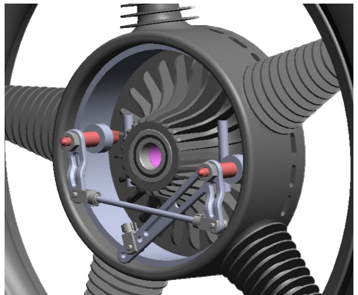
Monolithic Aluminum Wheel with Cooling Turbine - 2023
