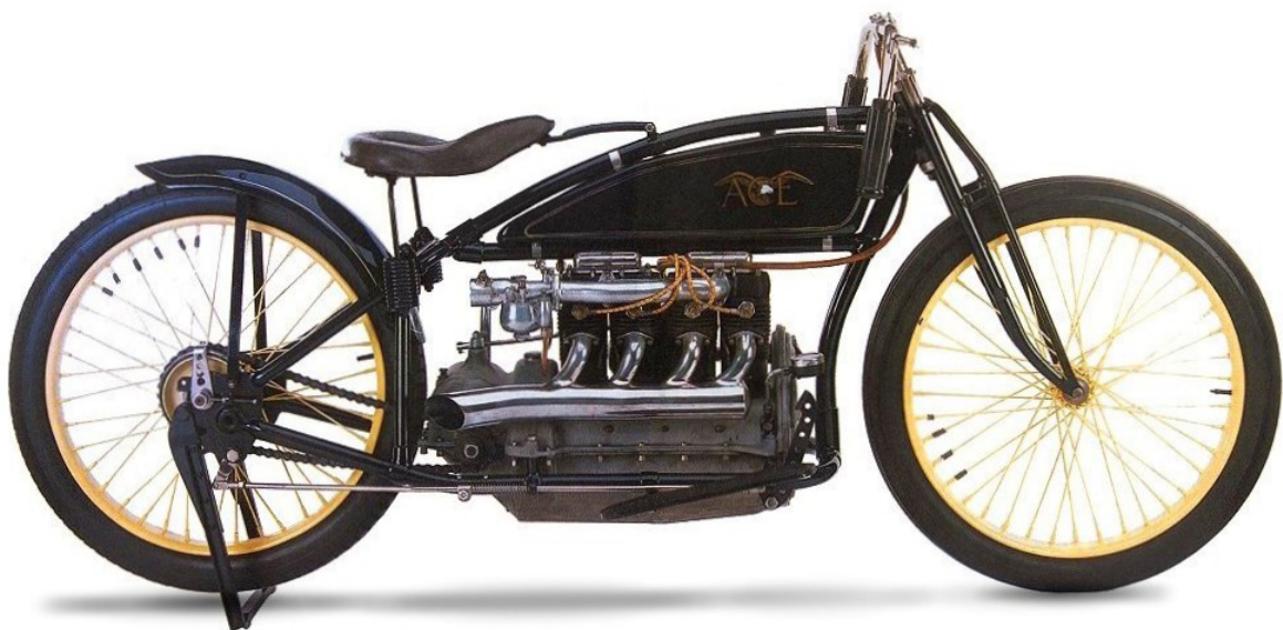
William Henderson's masterpiece, the 1923 Ace XP4
