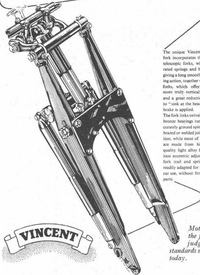
Vincent Girdraulic Front Suspension
