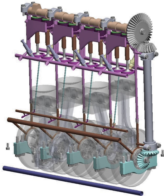
Oiling System
