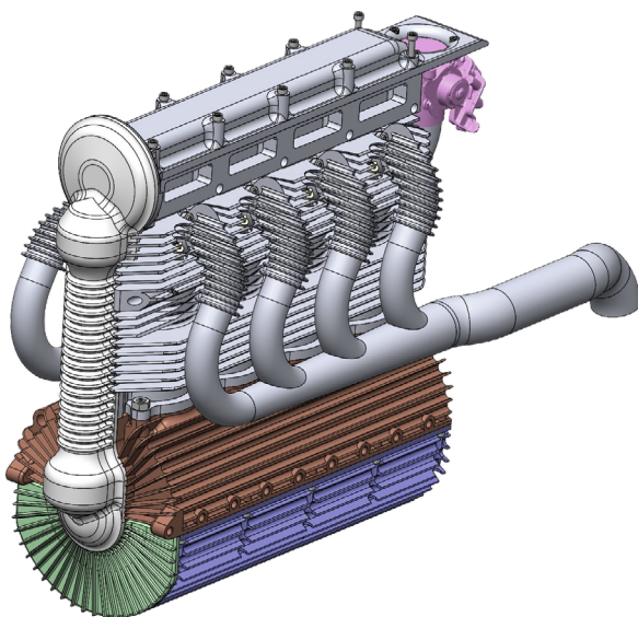
Engine CAD - 2023
