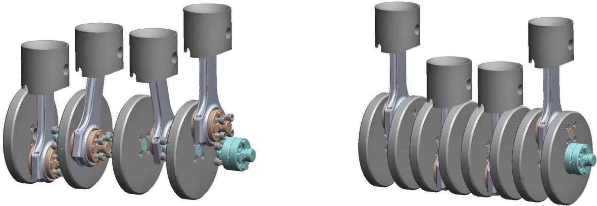
Configurable Crankshaft
